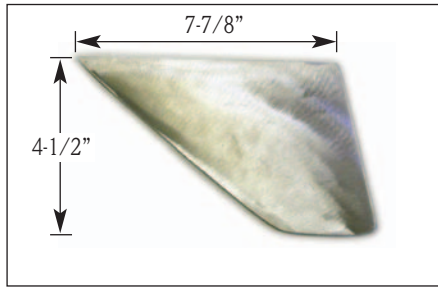
Yamaha 50 H.P. (Swept Back) Part No. SK17
