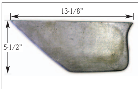
Mercury TR 215, Mercruiser III TRS Part No. SK11
