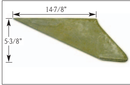
OMC 275 V-8 Part No. SK10
